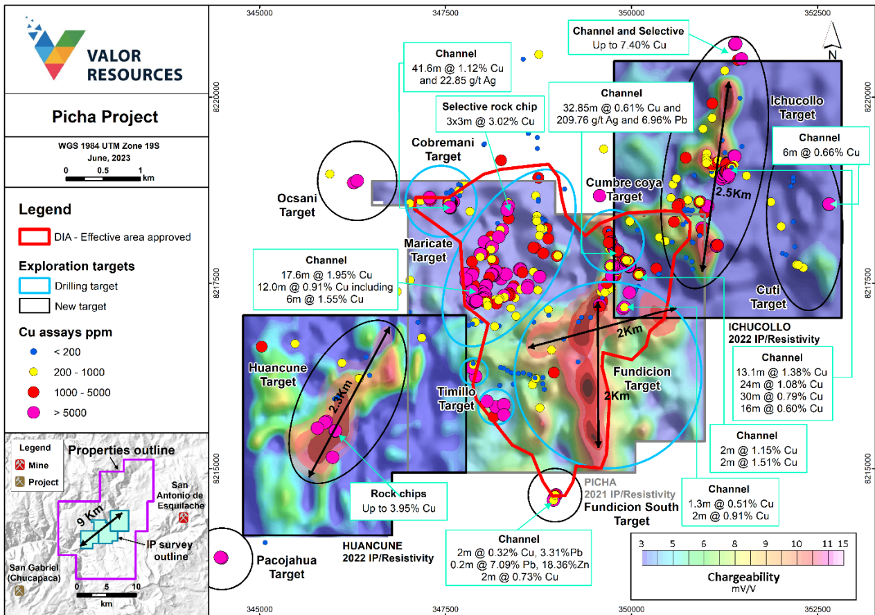
Figure 1: Picha Project – Drill targets, DIA approved area, surface geochemistry with Cu assays (overlaid on IP chargeability image)
